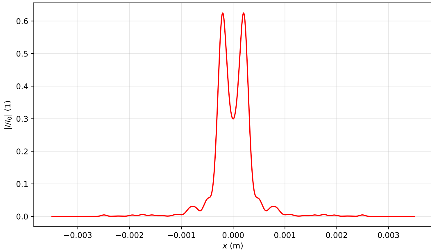
Intensity profile I(x, y = 0, z = 1.433)/I_0 , P_{in}=4.0P_{cr} , artificial time
